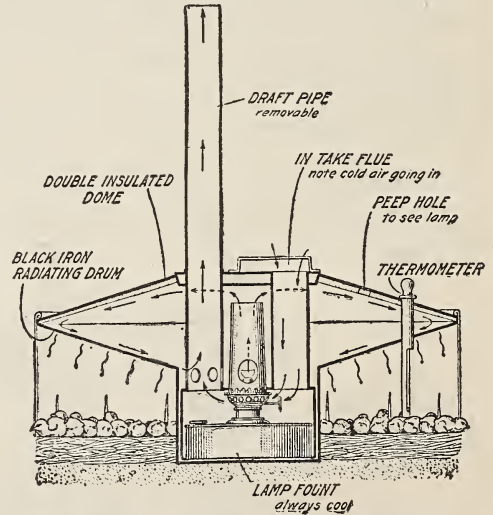
Sectional View of the Sanitary Hover
